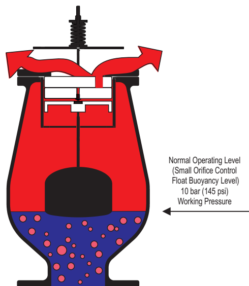
PRESSURIZED AIR/GAS RELEASE PIPELINE OPERATING
