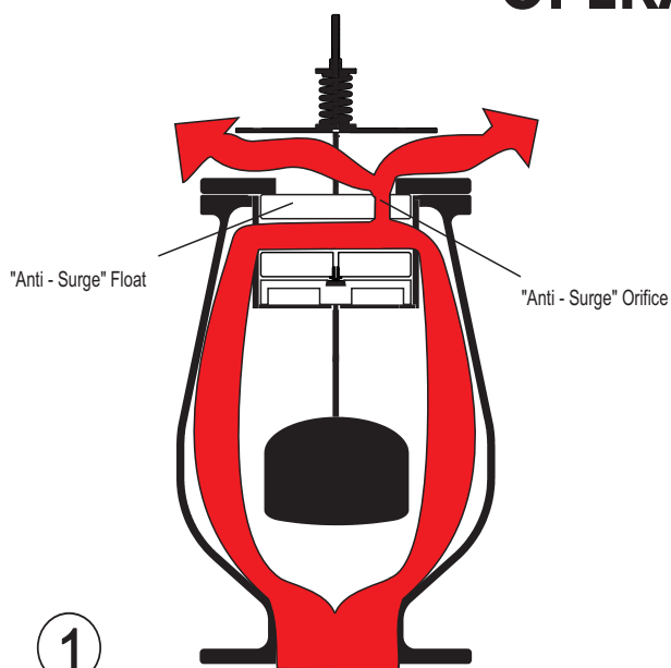
PIPELINE FILLING (SUB CRITICAL AND EXCESSIVE SEWAGE/ EFFLUENT APPROACH VELOCITY)
