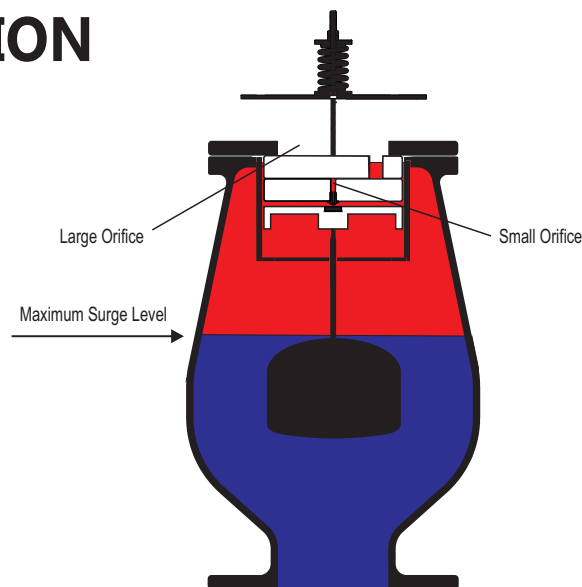
PIPELINE FULLY CHARGED
